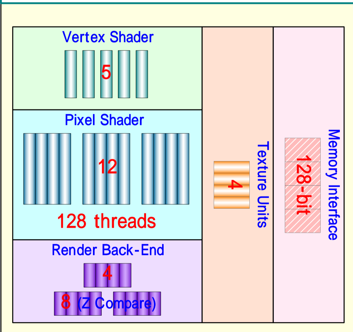
RADEON X1600 (RV530)
